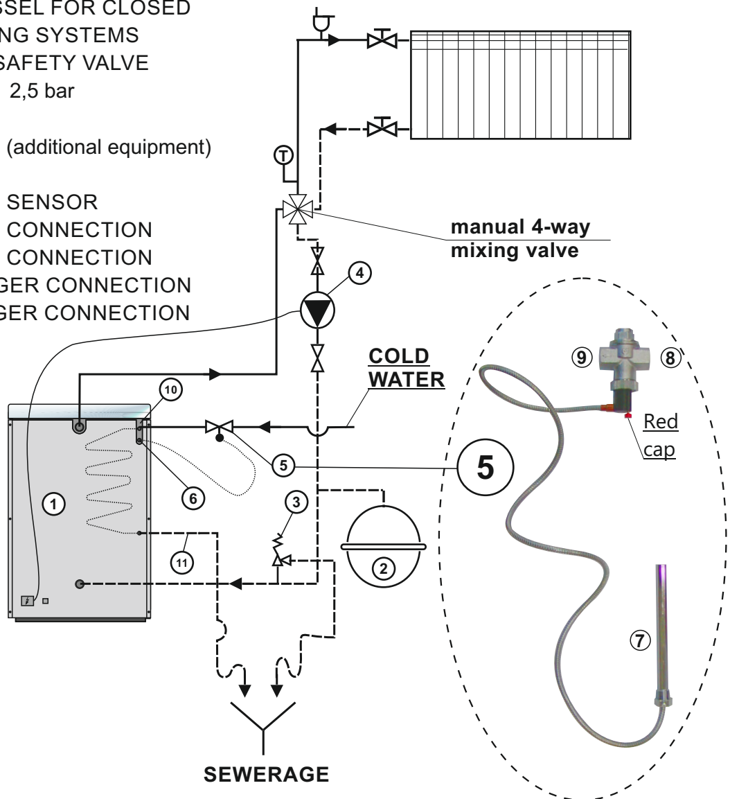
Diagram 2. - Connecting an BIO-CET 17 B
