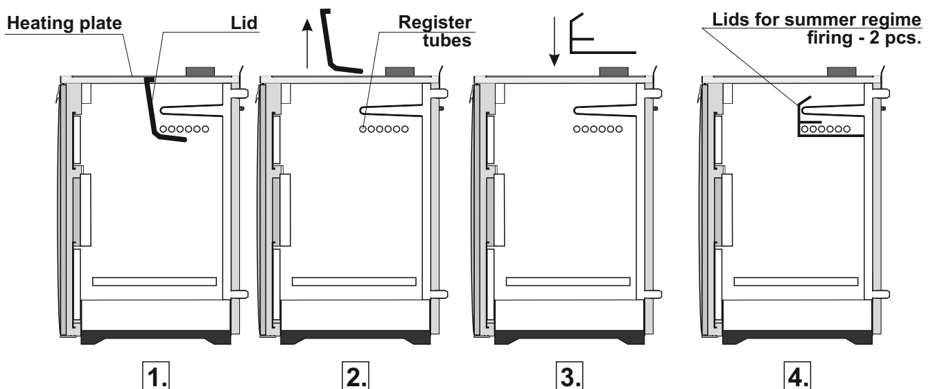
Image 4. - Installation of element for summer mod firing
